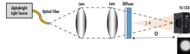
Figure 6. Lab test setup to characterize diffusers in converging and collimated beams.
